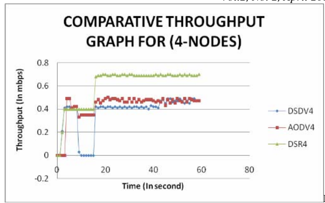
g. 2: Throughput Comparison for 4-nodes
