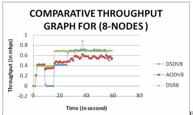
. 3: Throughput Comparison for 8-nodes
