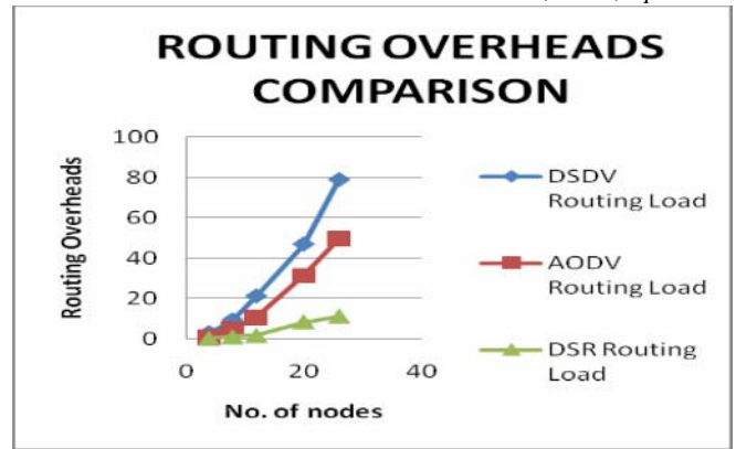
Fig. 8 Routing overheads for DSDV, AODV and DSR
