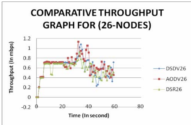
Fig. 6: Throughput Comparison for 26-nodes
