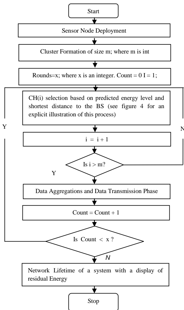
Fig 3 Flowchart of the Proposed Hierarchical Technique transfer with the employment of energy balancing technique for selection of CH via any shortest path to the
