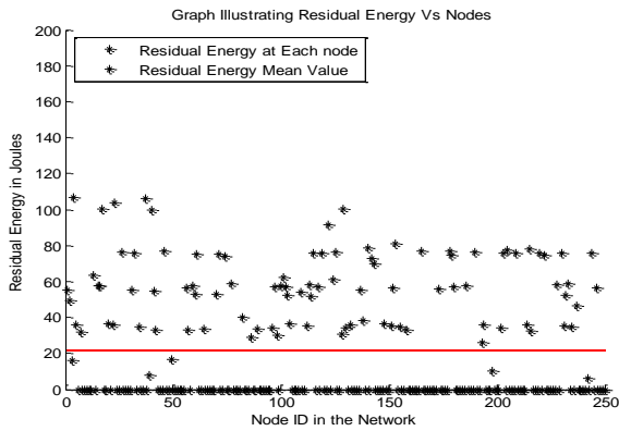
Fig 15: Nodes energy residue in second level hierarchical technique for five clusters after 400 round simulations.
