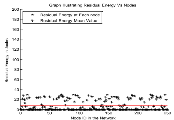
Fig 13: Nodes energy residue in first level hierarchical technique for three cluster after 400 round simulation
