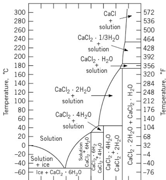
Fig-Phase diagram for the binary \text{CaCl}_2 - \text{H}_2\text{O} system
