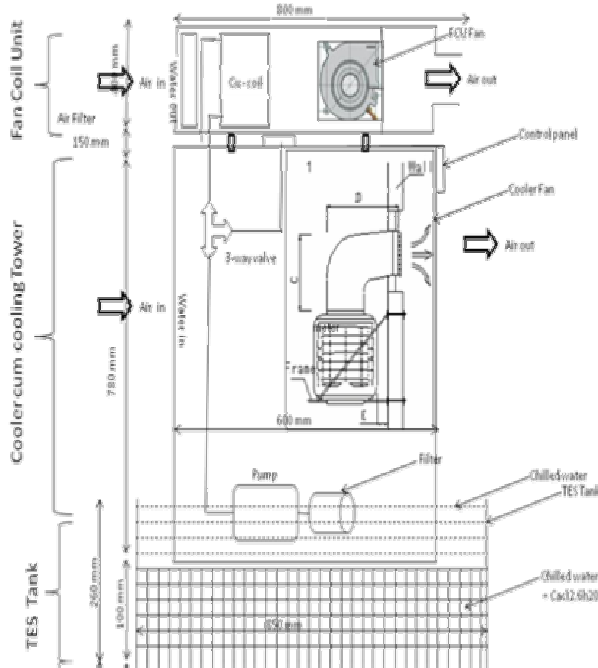
Fig – \text{CaCl}_2 \cdot 6\text{H}_2\text{O} based TES System for active building cooling purpose
